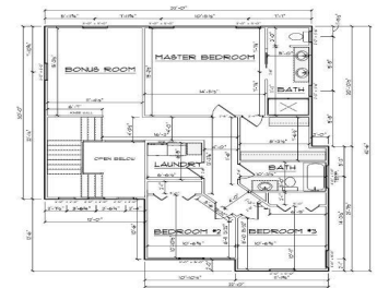
SECOND FLOOR - 1108 SQFT.
