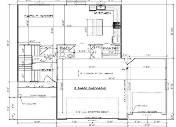
MAIN FLOOR - 786 SQFT.
