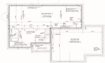
FOUNDATION PLAN SCALE 1/4" = 1'-0"
