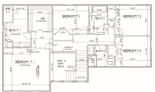
SECOND FLOOR PLAN SCALE 1/4" = 1'-0"
