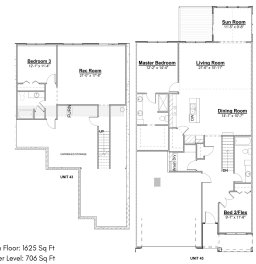
Main Floor: 1625 Sq Ft Lower Level: 706 Sq Ft Total: 2331 Sq Ft
