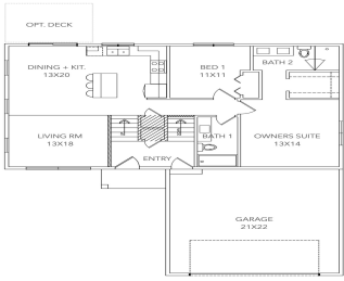
MAIN LEVEL
