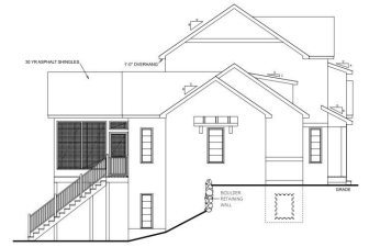
LEFT ELEVATION
